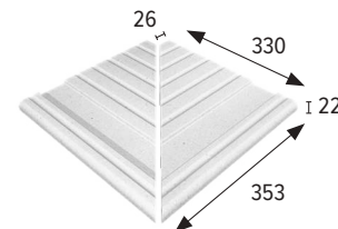
Esquina rejilla Corner grid**
