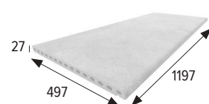
Borde monocompact 120 Monocompact edge 120
