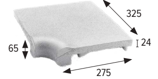
Remate esquina interior Internal corner
