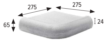
Remate esquina exterior External corner
