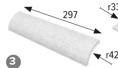
Cantонера External radial tile
